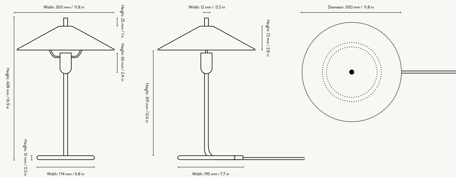
FRONT VIEW
