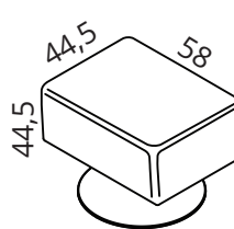
F3 Round base L4 chair base, D45cm, aluminium without tilting function
